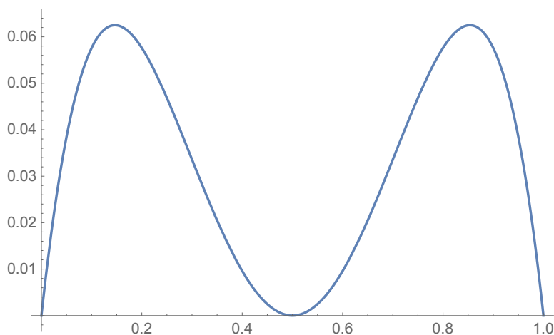
FIGURE 1. p(1-p)(1-2p)^2 as a function of p
